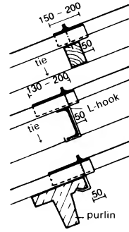
4 Fixing arrangements
